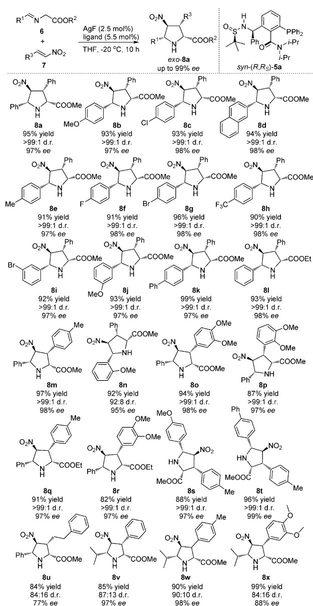
Scheme 3. Substrate scope of the synthesis of optically pure nitro-substituted pyrrolidines
