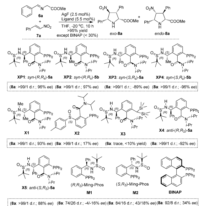
Scheme 2. Various chiral P-ligands for the silver-catalyzed cycloaddition of 6a and 7a . Reaction results are shown in parentheses.
