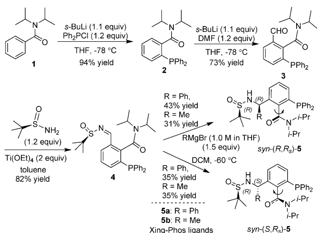
Scheme 1. Stereodivergent preparation of a new class of non-biaryl atropisomers with a phosphine group and multiple stereogenic centers.
